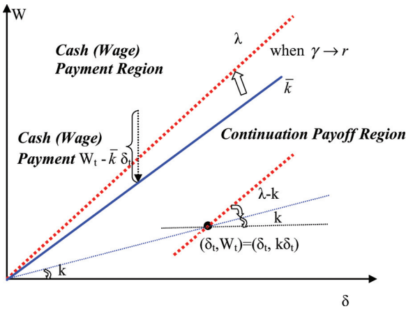
Figure 1 The optimal cash (wage) payment and incentive provision policy
