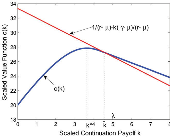
Figure 2 The scaled value function c(\cdot) for the case \gamma > r (an impatient agent) Parameters are r = 4\% , \gamma = 5\% , \mu = 1\% , \sigma^2 = 10\% , \lambda = 5 , L = 20 . \bar{k} < \lambda is a reflecting barrier. c(\cdot) attaches \frac{1}{r-\mu} - \frac{\gamma-\mu}{r-\mu}k with a slope -1 , and is extended for k > \bar{k} with a slope -1 .
