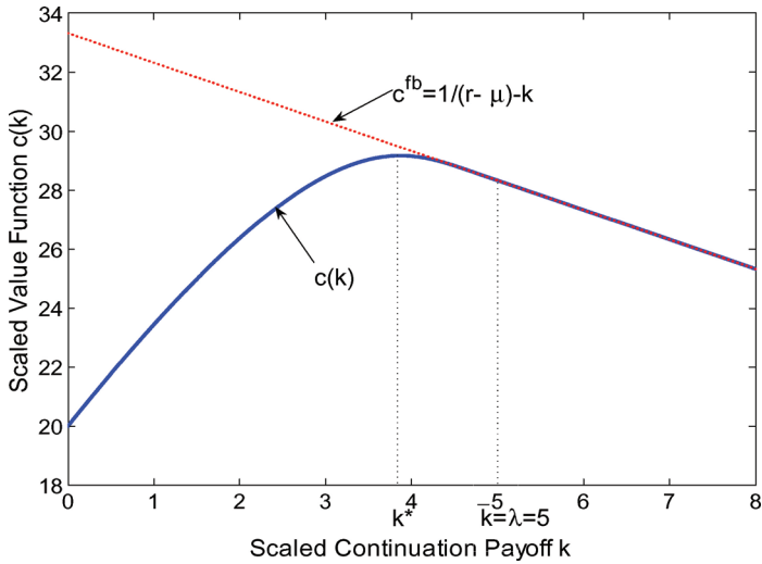
Figure 3 The scaled value function c(\cdot) for the case \gamma = r (an equally patient agent) Parameters are r = 4\% , \mu = 1\% , \sigma^2 = 10\% , \lambda = 5 , L = 20 . The scaled value function c(\cdot) attaches c^{fb}(k) = \frac{1}{r-\mu} - k smoothly, and \bar{k} = \lambda is an absorbing barrier.
